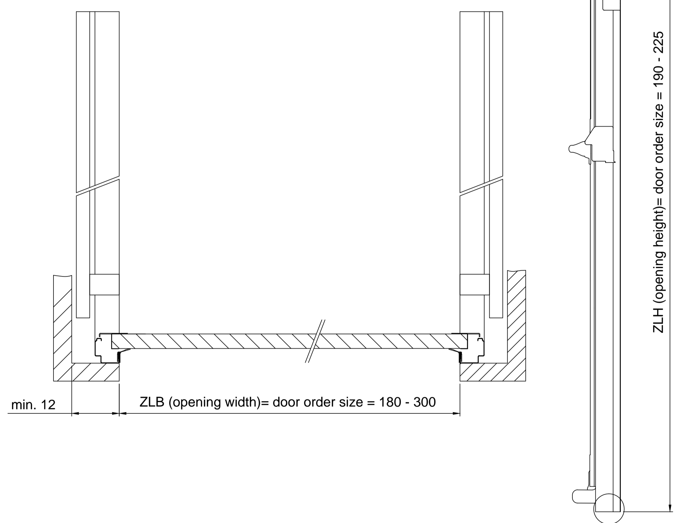
horizontal section
