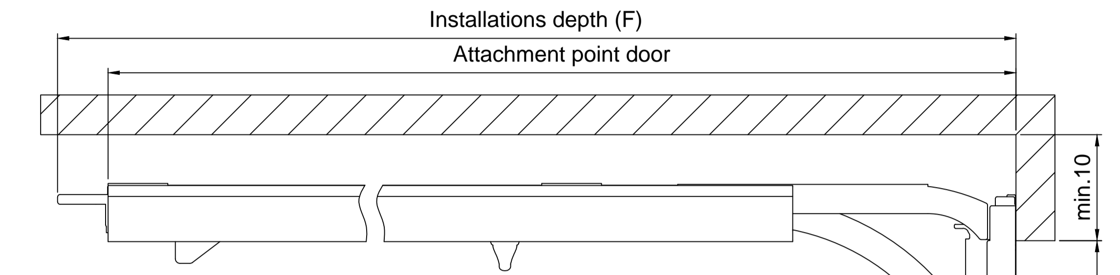
vertical section
