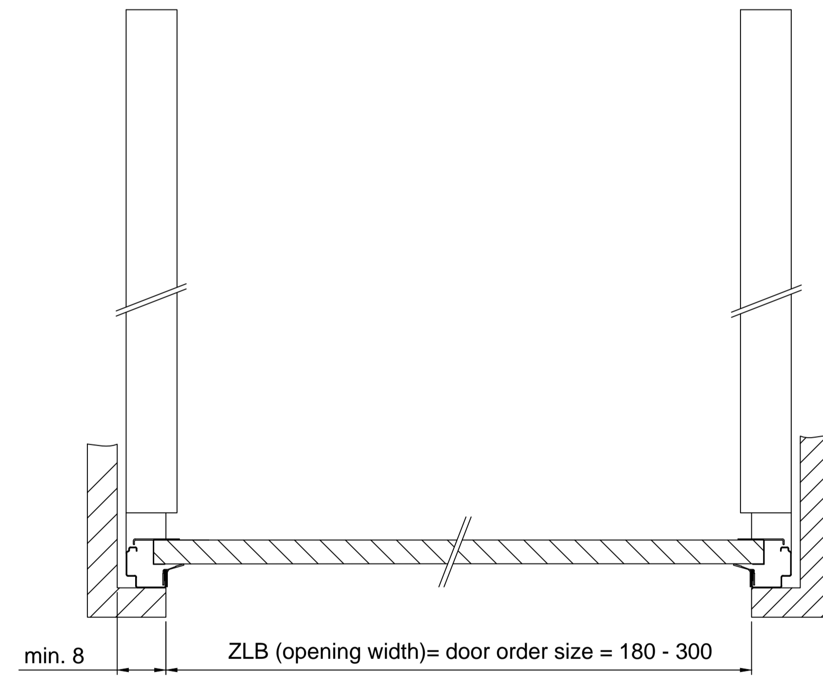
horizontal section
