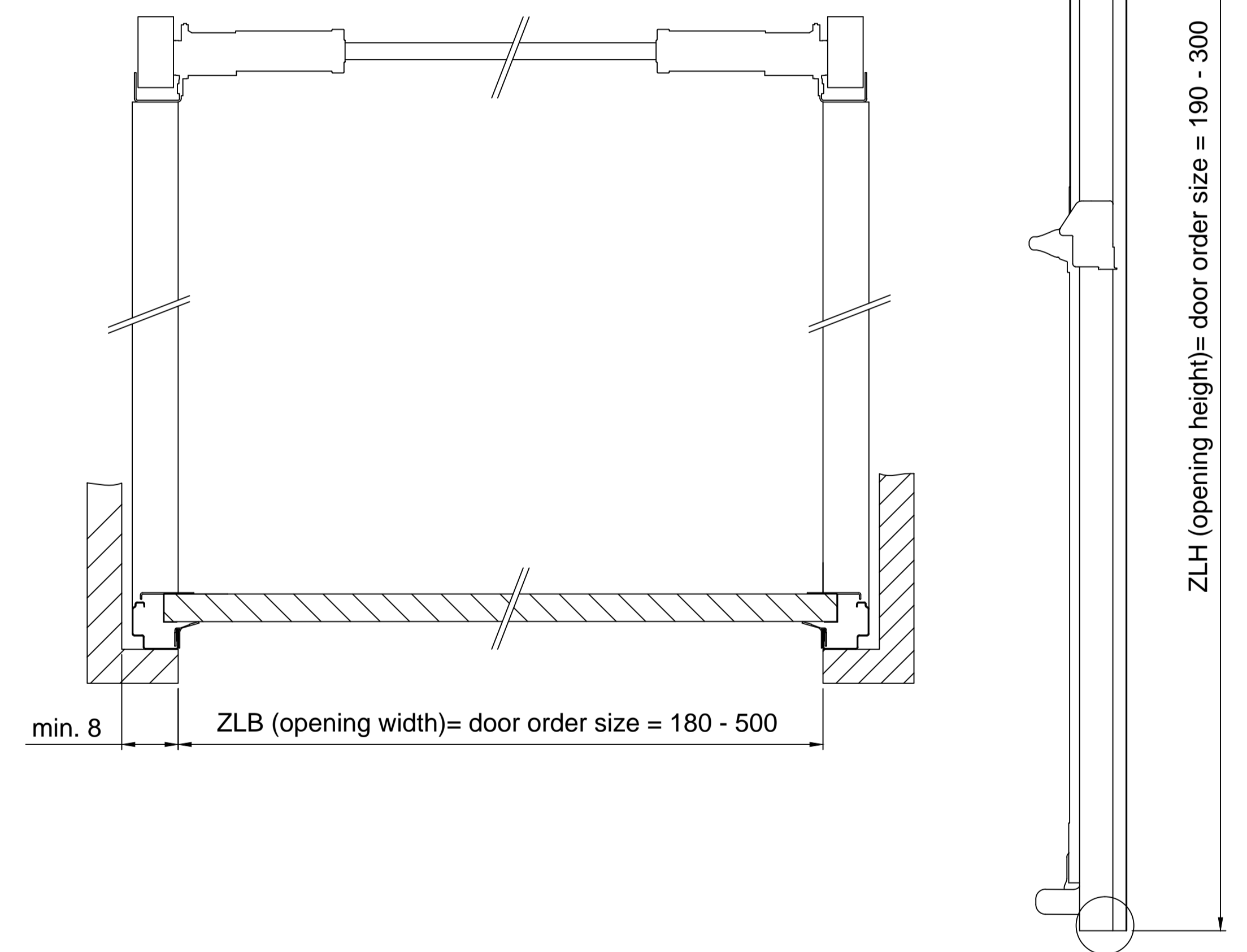
horizontal section
