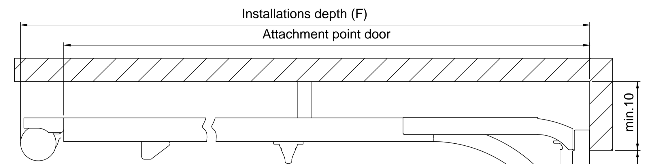
vertical section
