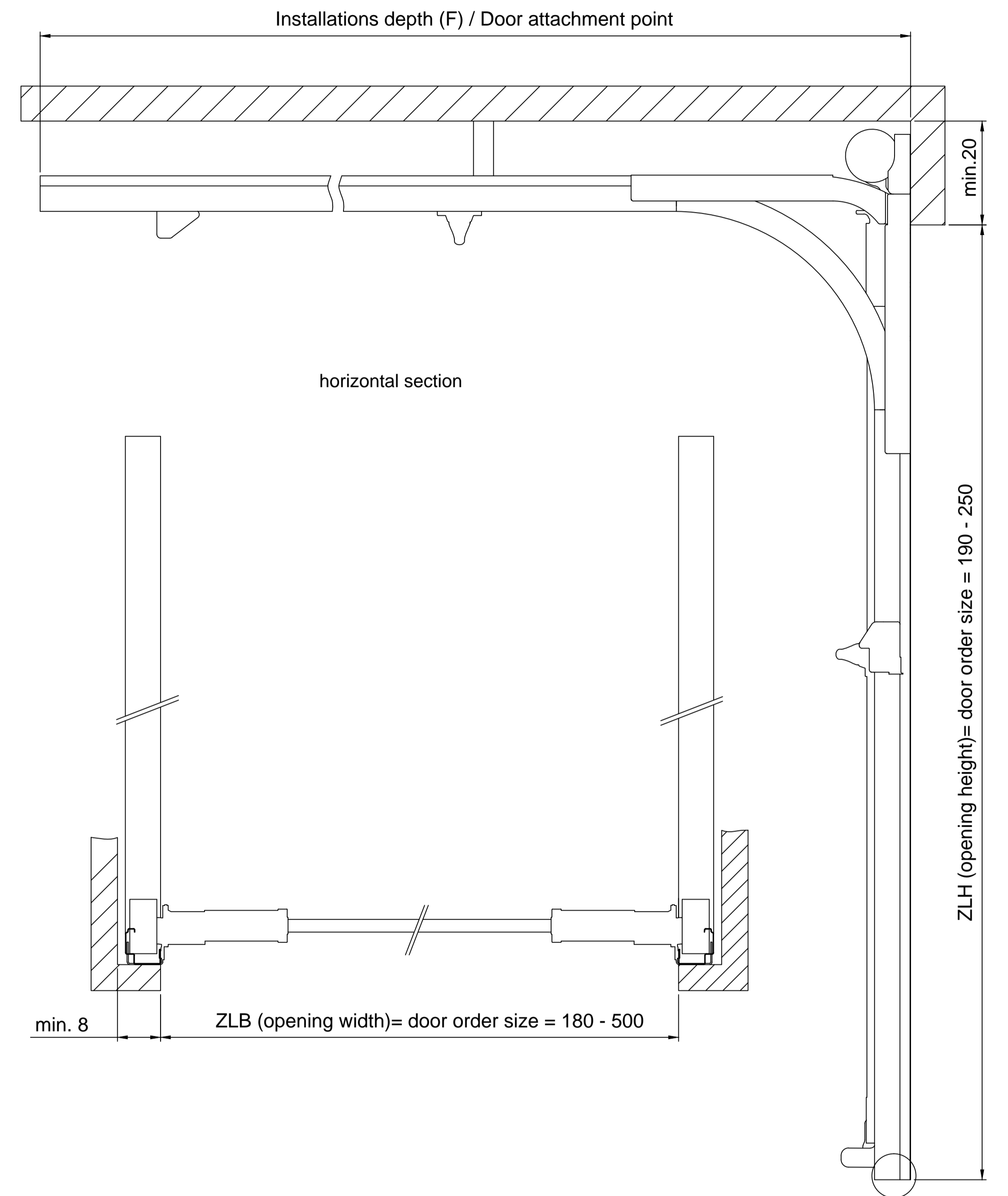
vertical section
